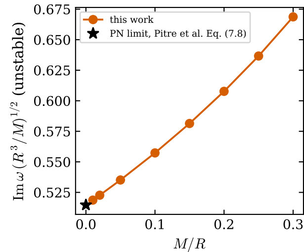
Even-parity matter modes of the static fluid shell (model C), \ell = 2 , \Gamma = 2 -- compare Pitre, Schneider & Poisson (2026) Figs. 1, 2
