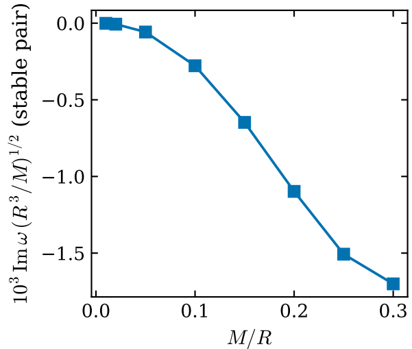
Even-parity matter modes of the static fluid shell (model C), \ell = 2 , \Gamma = 2 -- compare Pitre, Schneider & Poisson (2026) Figs. 1, 2
